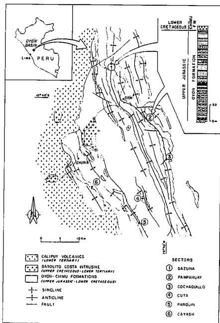
Fig.1.- Geographical location and geological setting of the Oyón Basin (Peru).
